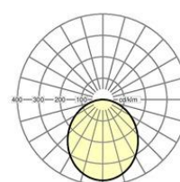
PNEG/600 IP 54 LED 4200 lm 840
