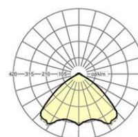
SDGSOXB LED 9000 lm 840
