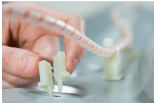
Rivet Mount TY5 is usable with a wide variety of our cable ties.
