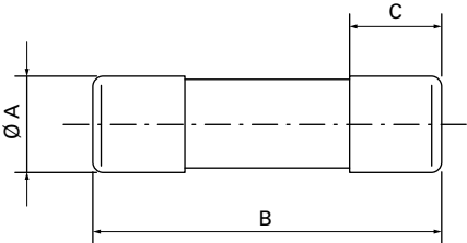
C22 Dimensions - mm
