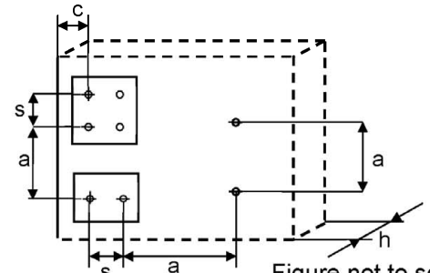
Scheme of edge distances and spacing in concrete base material group “a”
