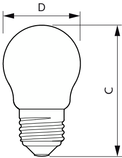
MASTER VLE LEDLusterDT3.5-40W E27 927P45FRG
