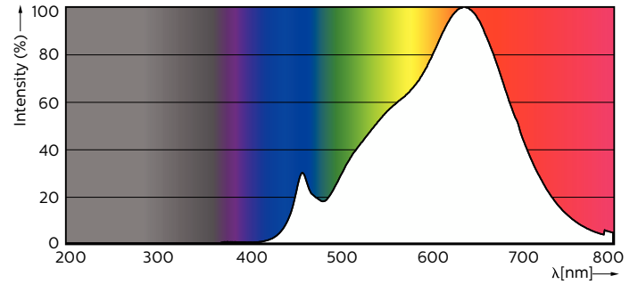
Accent Lighting Spots - MAS LED ExpertColor 3.9-35W GU10 927 36D Spectral Power Distribution Colour - MAS LED ExpertColor 3.9-35W GU10 927 36D
