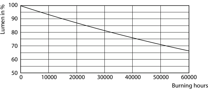
Lumen Maintenance Diagram - TForce LED HPL ND 57-42W E27 830
