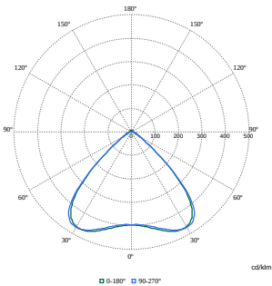
Polar Normal (separate) - WT490CI - 910925868287
