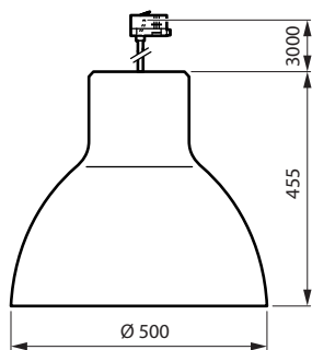
PT520T LED49S/830 PSU MB BELL CL
